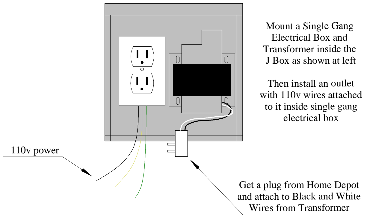
6" x 6" Exterior Junction Box with Outlet and Transformer
